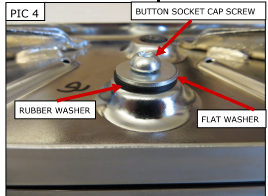
RUBBER MOUNTS IN HOLES
